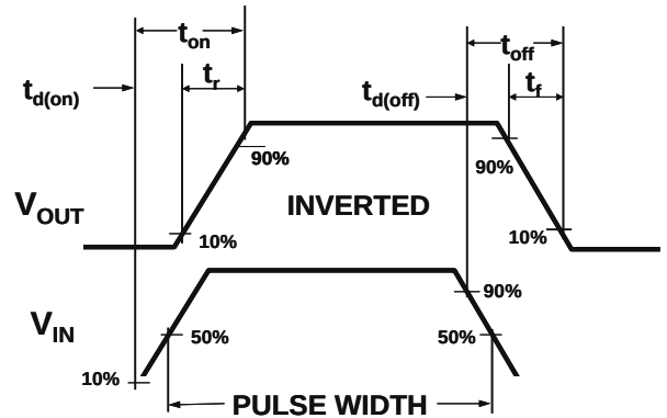
Figure 2: Switching Waveforms
