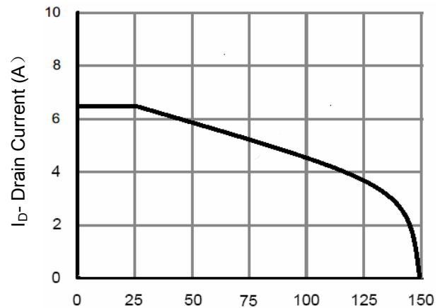
Figure 4 Drain Current
