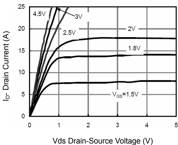
Figure 5 Output Characteristics
