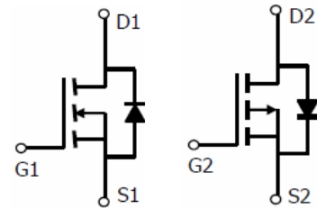
N-channel
