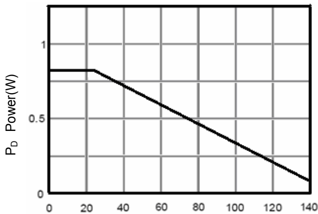
Figure 3 Power Dissipation
