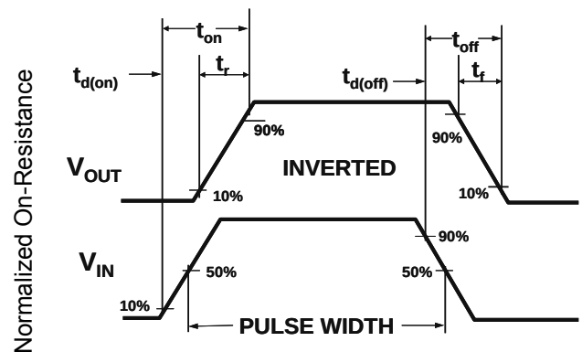
Figure 2: Switching Waveforms
