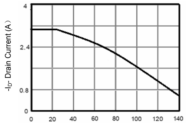
Figure 4 Drain Current
