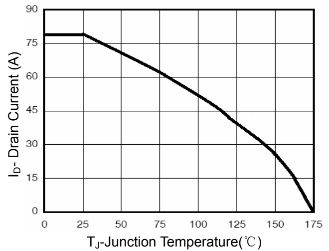
Figure 9 Current De-rating
