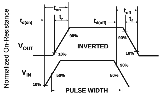
Figure 2: Switching Waveforms
