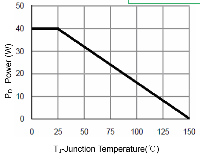
Figure 9 Power Dissipation
