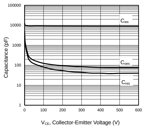
Figure 5 Capacitance Characteristics
