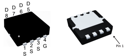
DFN3.3x3.3-8_EP
