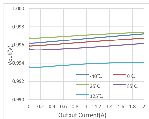
V_{IN} = 1.4\text{ V} , V_{OUT} = 1.0\text{ V} Output Voltage vs Output Current
