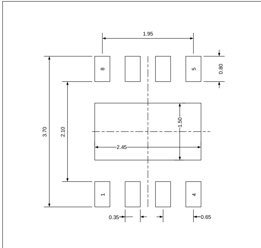
Figure 9-2 DFN8 recommend Footprint
