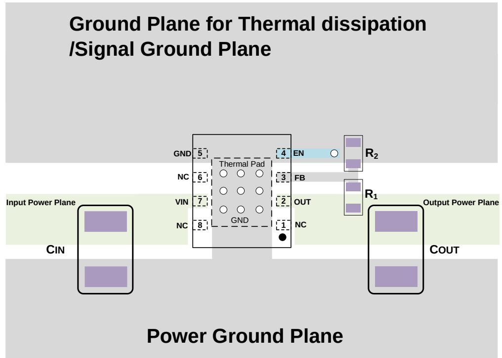
Figure 8-1 Typical GD30LD1002x layout guideline
