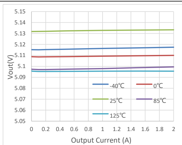
V_{OUT} = 5.1\text{ V} Output Voltage vs Output Current
