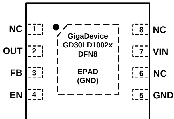
Figure 4-2 GD30LD1002x DFN8 pinouts
