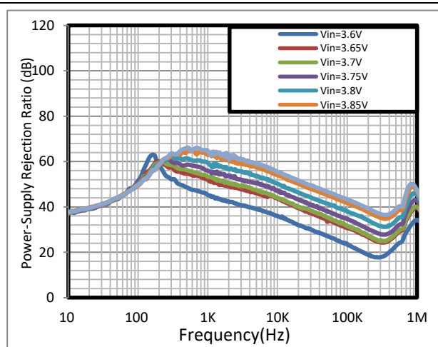
V_{OUT} = 3.3\text{ V} , I_{OUT} = 1.2\text{ A} C_{OUT} = 10\text{ }\mu\text{F} \parallel 10\text{ }\mu\text{F} , C_{FF} = 10\text{ nF} PSRR vs Frequency and V_{IN} for V_{out} = 3.3\text{ V}
