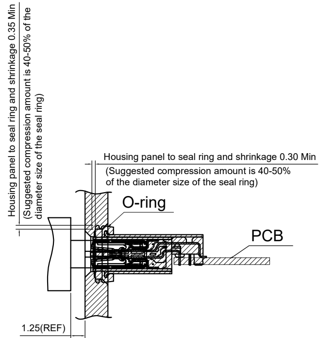
SCHEMATIC DIAGRAM OF PLUGGING THE MALE AND FEMALE HEADS AFTER ASSEMBLING THE PANEL
