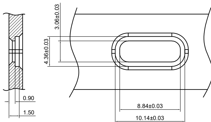
RECOMMENDED HOLE SIZE FOR THE CASE
