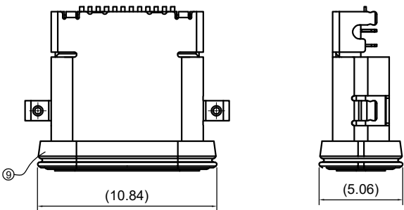
SCHEMATIC DIAGRAM OF ASSEMBLING THE WATERPROOF RING (CUSTOMER WILL ASSEMBLE IT AFTER MOUNTING THE BOARD)
