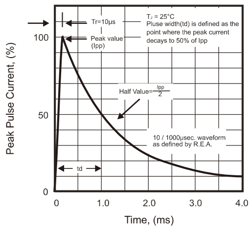
Fig.5 - Pulse Waveform
