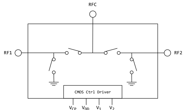
Figure 2: TS8023N functional diagram
