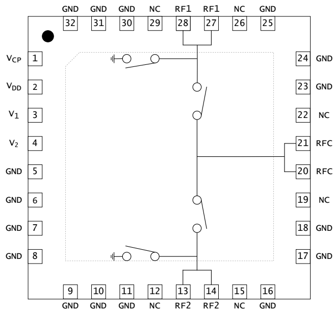
Figure 3: TS8023N pin assignment [top view]
