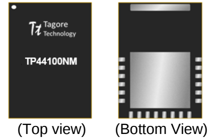
Figure 1 Device Image (22pin 5×7×0.85 mm QFN Package)
