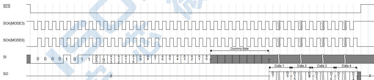
图 9 - 5: SPI Fast Read
