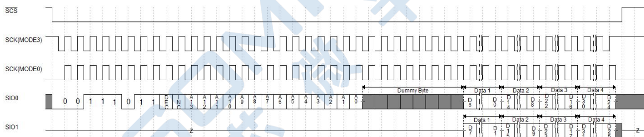
图 9 - 7: SPI Dual Output Read
