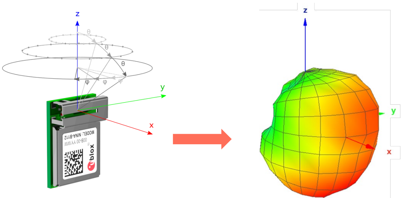
Figure 5: Measurement procedure for determining radiation patterns
