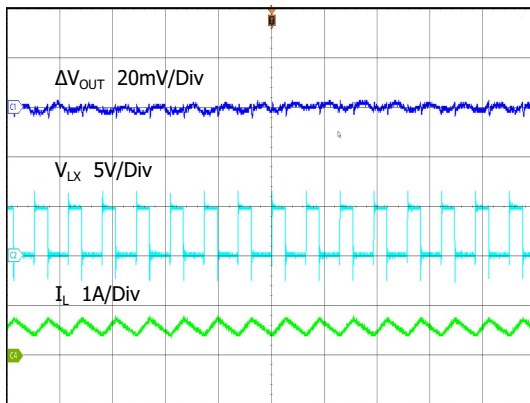
Output Ripple
