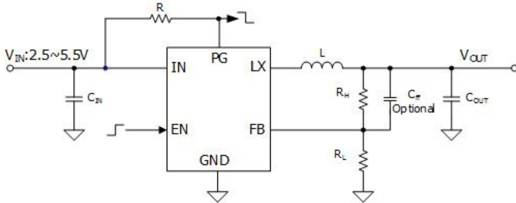
WD3410 Basic Application Circuit
