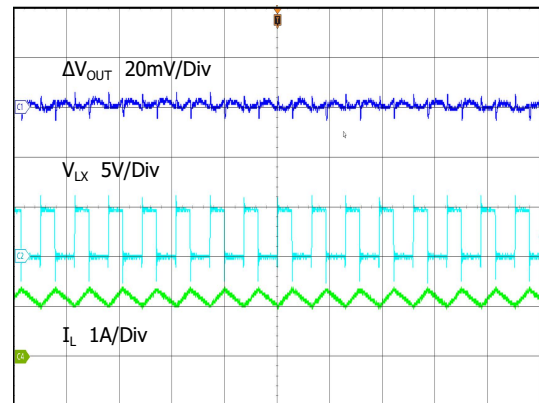
Output Ripple
