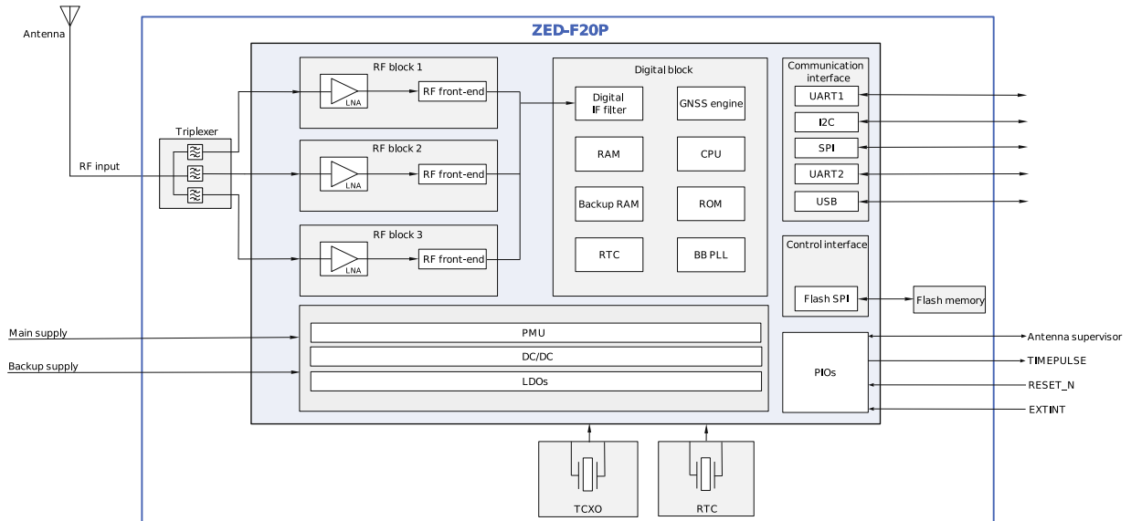
Figure 1: ZED-F20P block diagram
