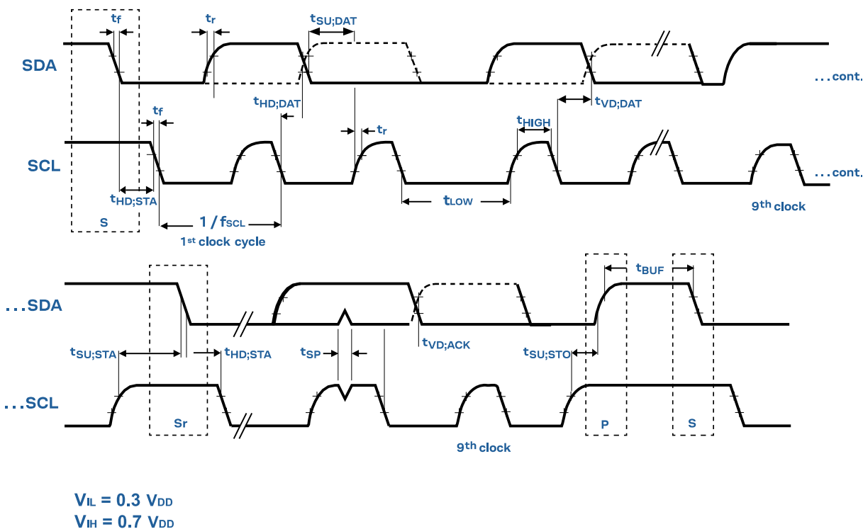
Figure 4: ZED-F20P I2C peripheral specification
