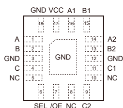
QFN2.8x2.0-18L
