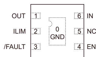
TDFN2x2-6L
