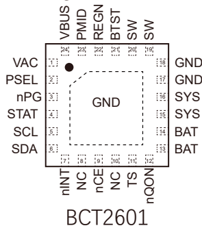
QFN4x4-24L
