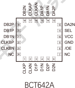
QFN3.4x2.5-24L
