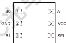
DFN1x1-6L DFN1.1x0.9-6L TDFN1.1x0.9-6L
