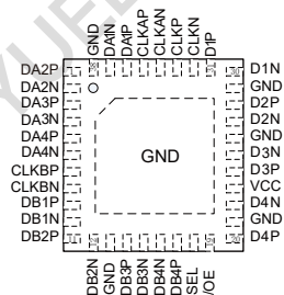
QFN4x4-38L
