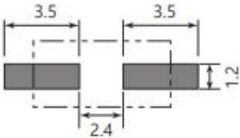
Land Pattern
