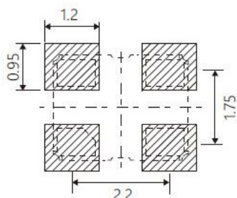
Land Pattern
