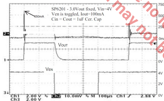
Fig. 30: Inrush Current, I_O=100\text{mA}
