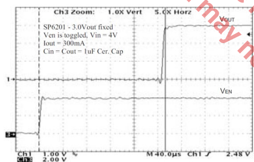
Fig. 24: Turn on time, I_O=300\text{mA} , 4V_{IN}
