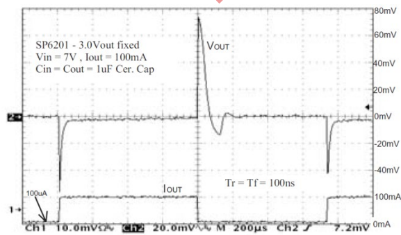
Fig. 33: Load Transient Response, 100mA step, 7V_{IN}
