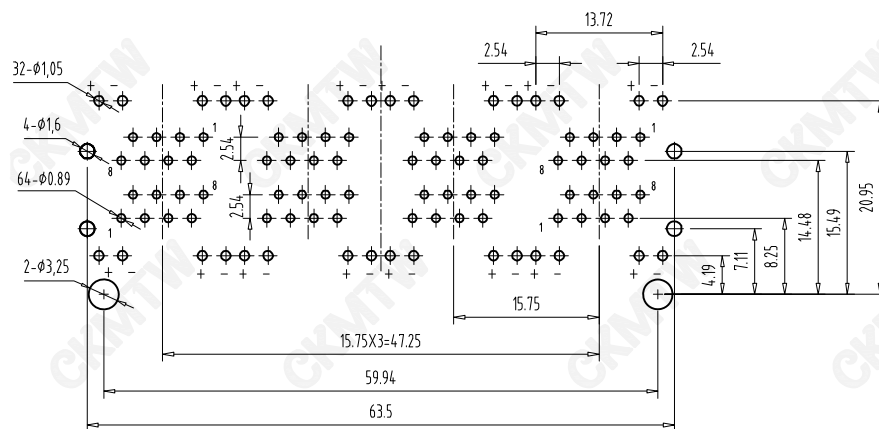
PC Board Layout Component Side Shown
