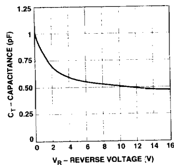
Figure 15. Total Capacitance vs. Reverse Voltage—HSMS-2810 Series.
