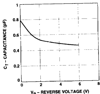
Figure 16. Total Capacitance vs. Reverse Voltage—HSMS-2820 Series.
