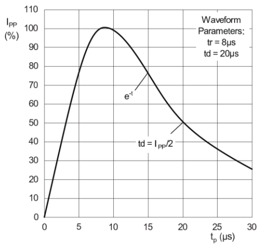
Figure 3 Pulse waveform
