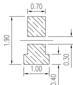
METAL MASK T=0.10 TOLERANCE: ±0.05 (钢网推荐图)
