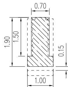
RECOMMENDED PCB LAYOUT TOLERANCE: ±0.05 (焊盘推荐图)
