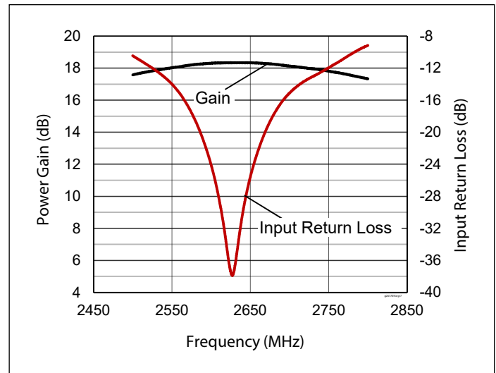
Figure 12. Small Signal CW Performance
