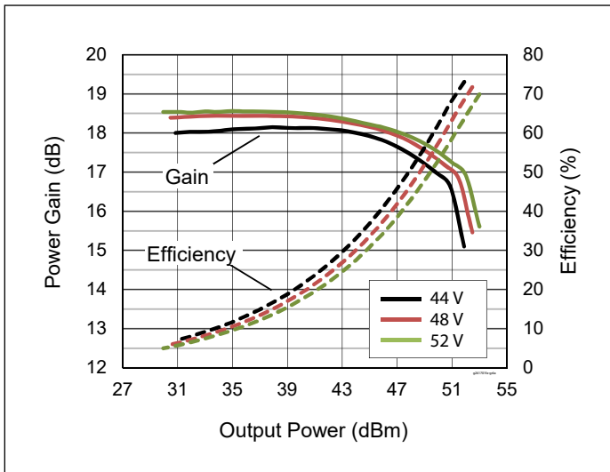
Figure 9. CW Performance at Specified V_{DD}
