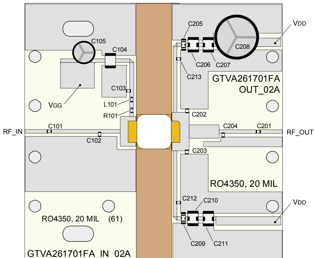
Reference circuit assembly diagram (not to scale)
