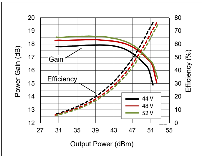
Figure 11. CW Performance at Specified V_{DD}
