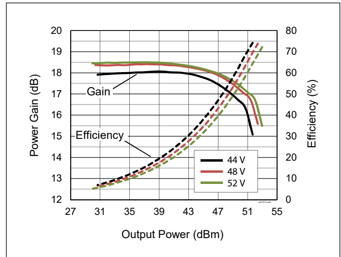
Figure 10. CW Performance at Specified V_{DD}
