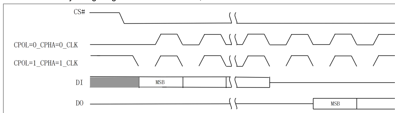
Figure 7.1 SPI Modes
