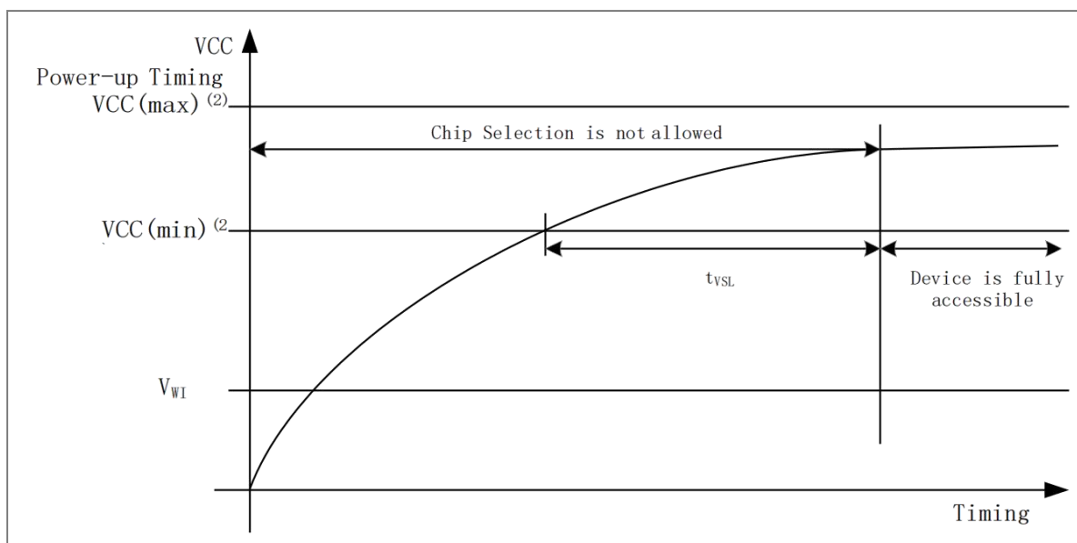
Figure 9.1 Power-up Timing
