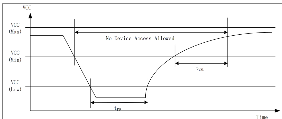
Figure 9.2 Power-Down and Voltage Drop
