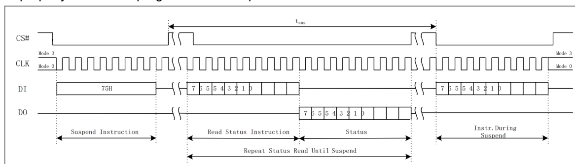
Figure 8.11a Erase / Program Suspend Instruction(SPI Mode)
