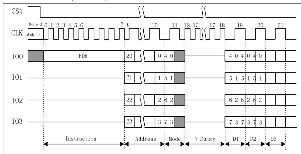
Figure 8.22a DTR Fast Read Quad I/O Instruction (M7-0 = FFh, SPI Mode)
