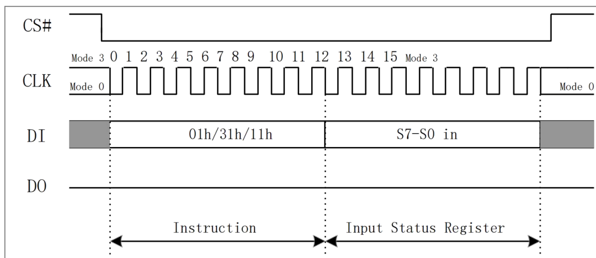
Figure 8.5a Write Status Register Instruction(SPI Mode)
