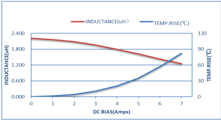
ZEPIM303012D-2R2M
