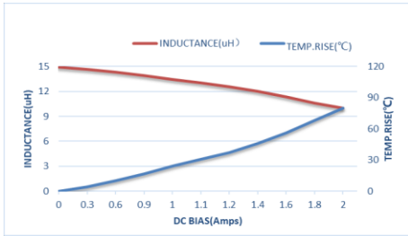
ZEPIM303012D-150M
