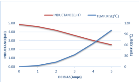
ZEPIM303012D-4R7M
