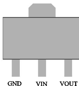
SOT89 A (Top view)
