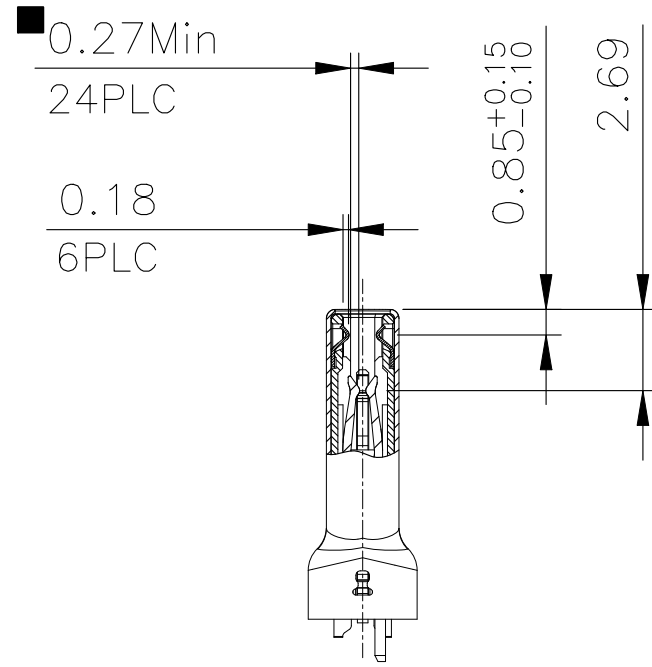
SECTION B-B SCALE 1:1 (WITH EMI SPRING)
