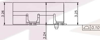
SECTION B-B SCALE 1:1
