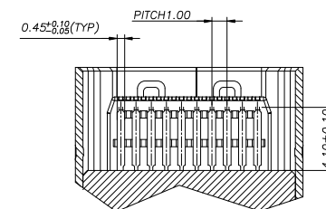
SECTION: B-E
