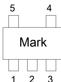
SOT-23-5L (Top View)
