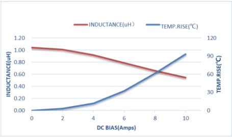
ZET-CORE-303012DT1R0MBCA
