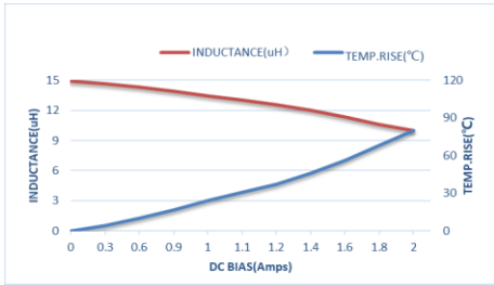
ZET-CORE-303012DT150MBCA
