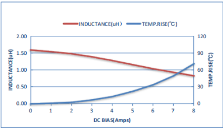
ZET-CORE-303012DT1R5MBCA
