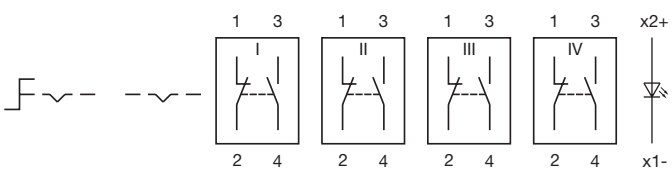
Wiring diagram 280
