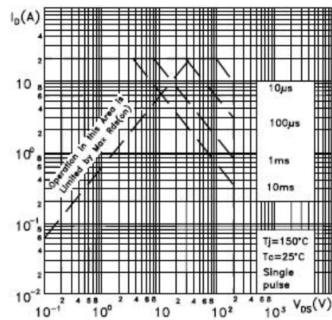
Fig6 Maximum Safe Operating Area
