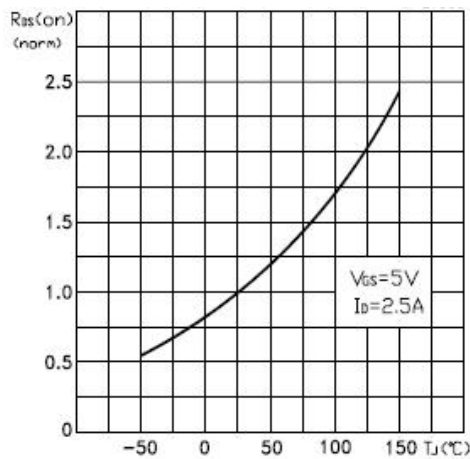
Fig3 Normalized On-Resistance Vs. Temperature
