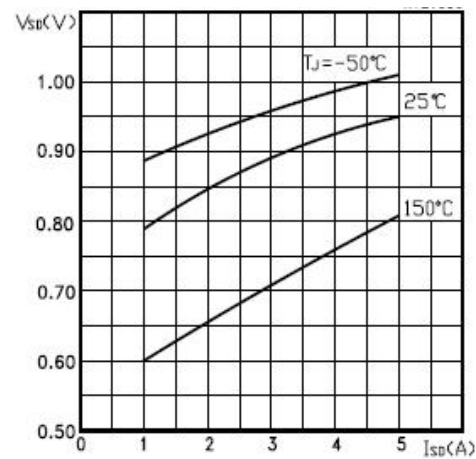
Fig4 Typical Source-Drain Diode Forward Voltage
