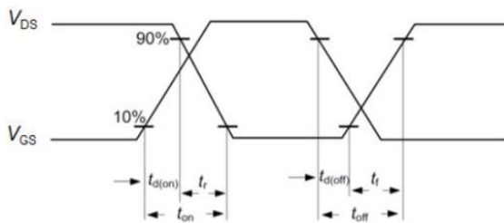
Figure A. Definition of switching times
