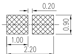
METAL MASK T=0.08
