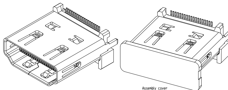
Assembly cover
