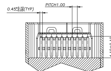
SECTION-B
