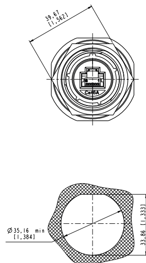
Panel drilling
