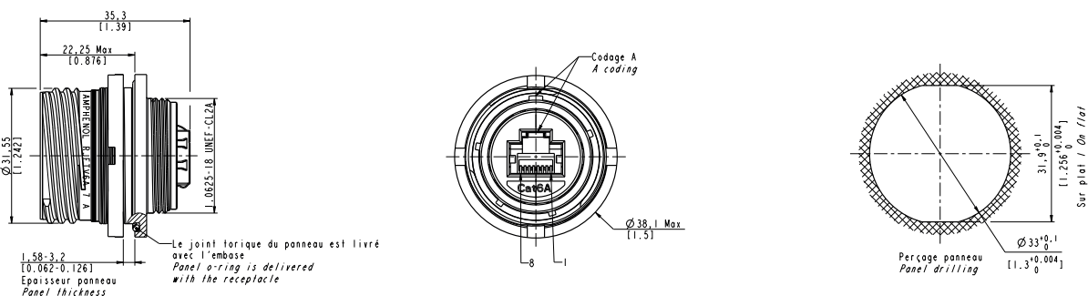
Panel drilling
