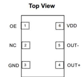
Figure 1. Pin Assignments
