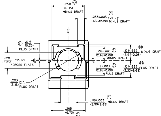
DETAIL E
