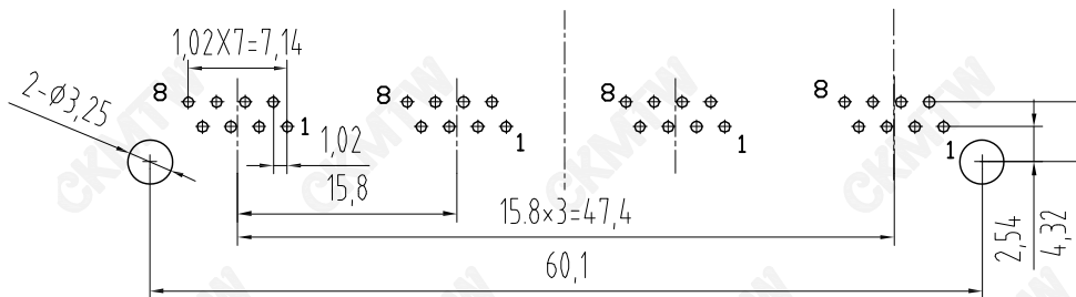
PC Board Layout Component Side Shown
