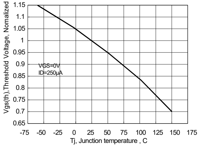
Figure 10 Typical Theshold Voltage vs Junction Temperatur
