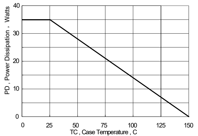
Figure 2 Maximum Power Dissipation vs Case Temperature 14
