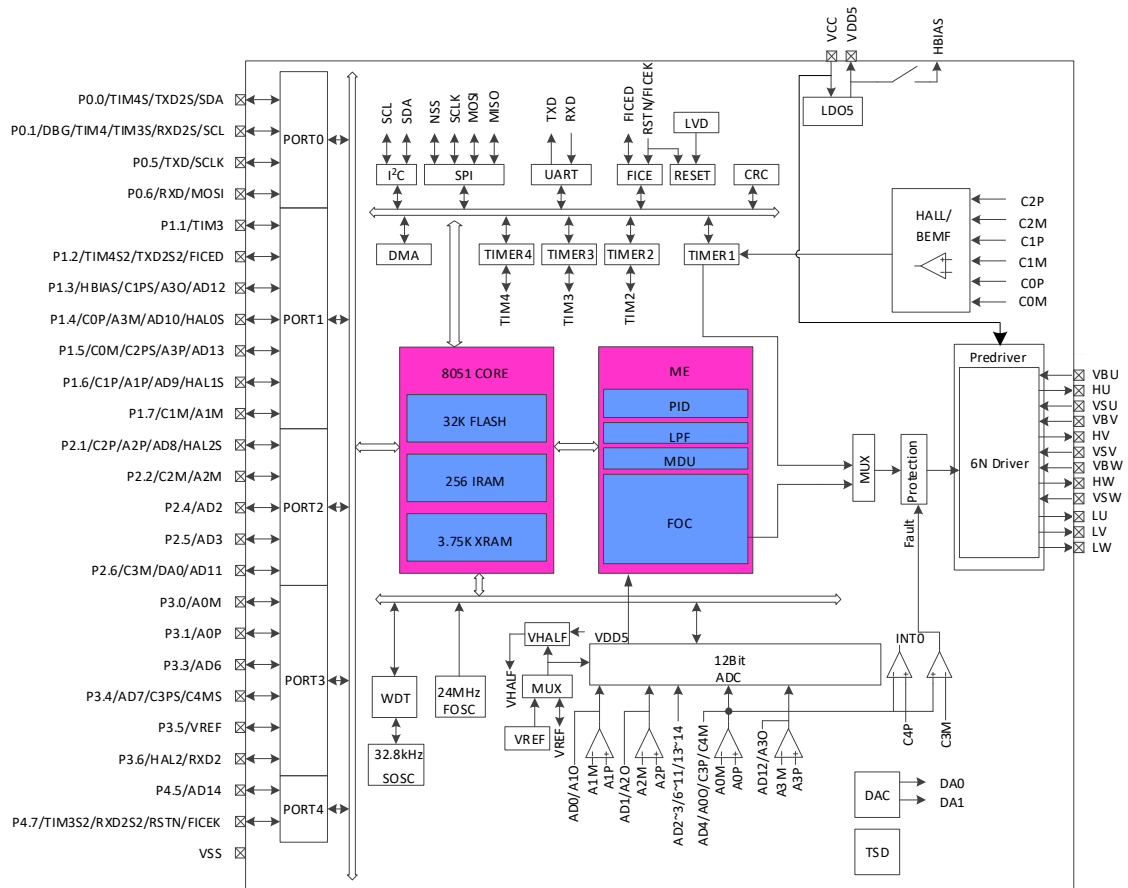
Figure 1-2 Functional Block Diagram of FU6572N
