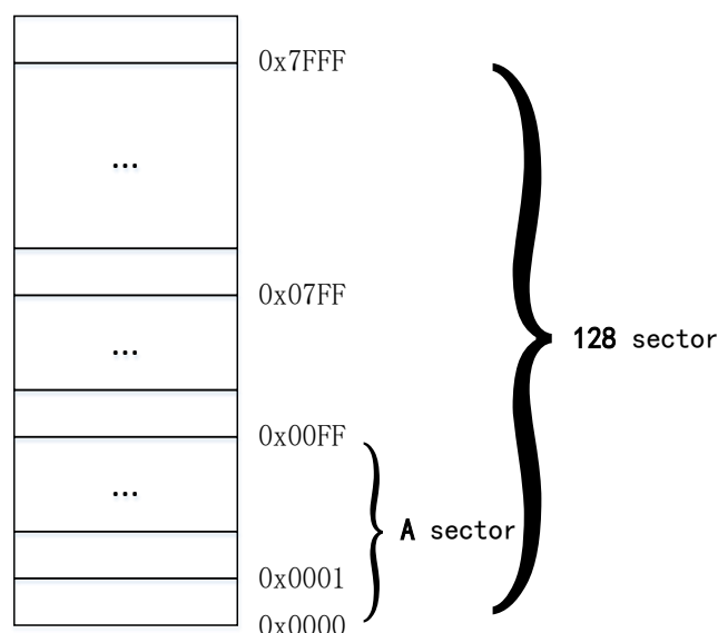
Figure 30-3 ROM Sectors
