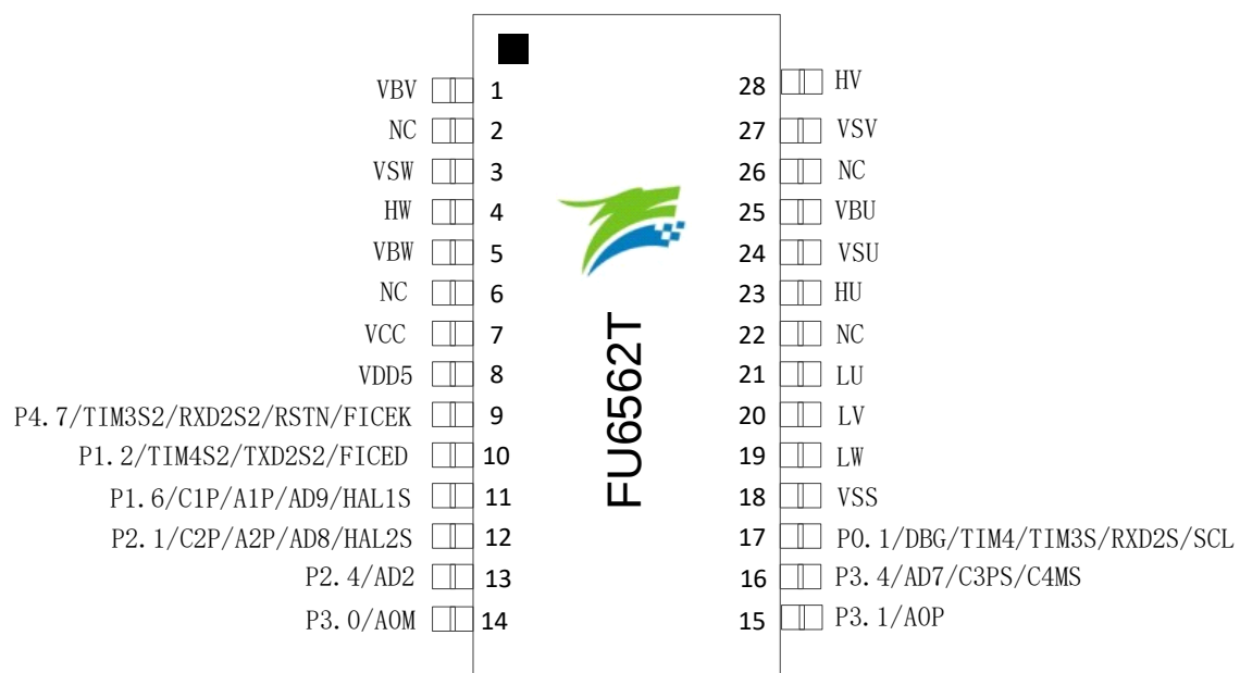
Figure 2-5 FU6562T TSSOP28LD Pinout Diagram
