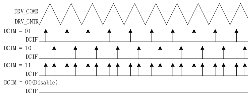
Figure 17-9 Driver Compare Match Interrupt
