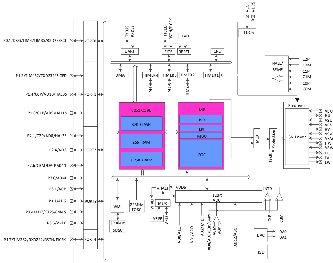
Figure 1-3 Functional Block Diagram of FU6572T
