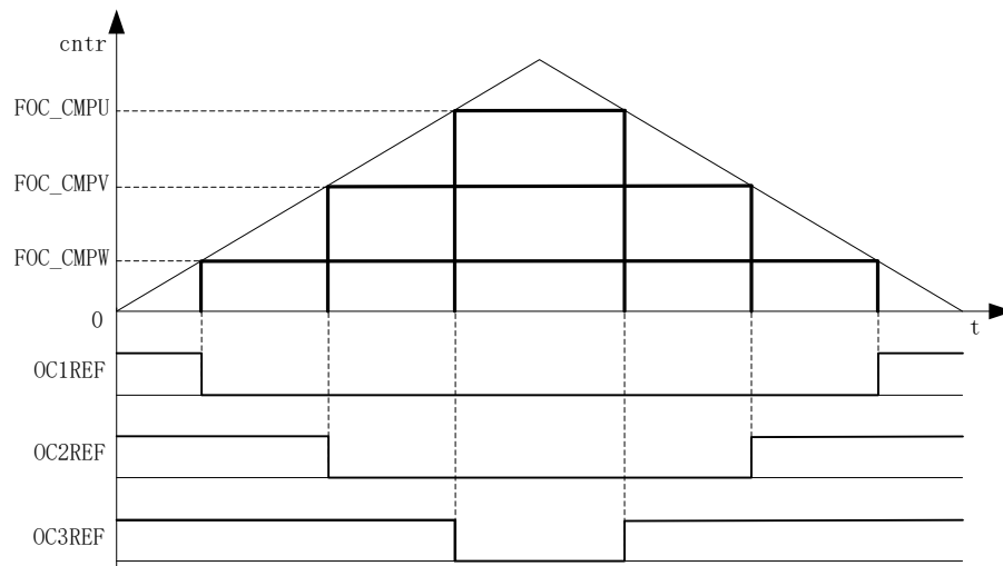
Figure 17-4 PMW Generation
