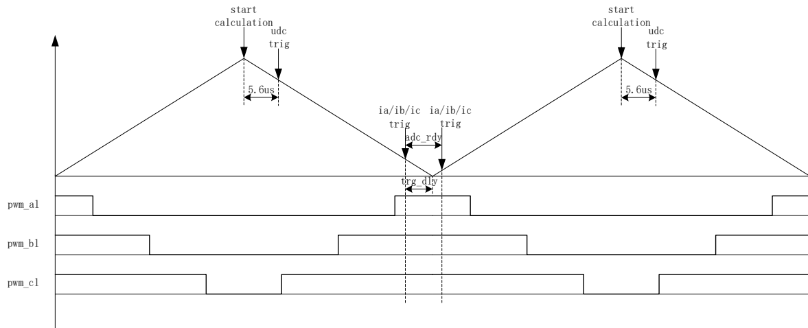
Figure 12-12 Dual/Triple-shunt Sequential Current Sampling Mode
