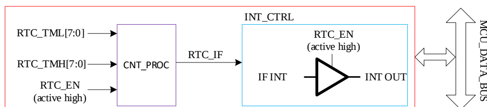
Figure 19-1 RTC Functional Block Diagram
