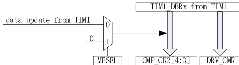
Figure 17-6 Timer1 Automatic Control of DRV_CM[R] and CMP_CR2[4:3]
