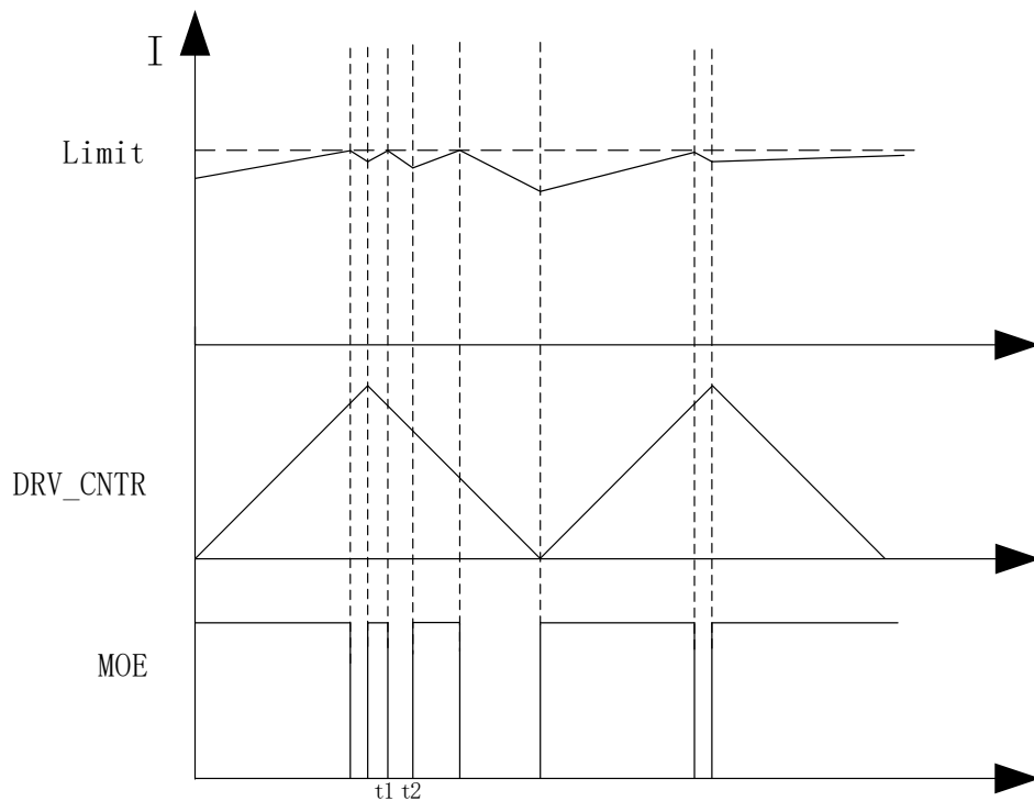
Figure 27-6 Cycle-by-cycle Current Limiting Waveform ( t_2 - t_1 = 5\mu\text{s} ) when \text{EVT\_FLT}[\text{MOEMD}] = 11
