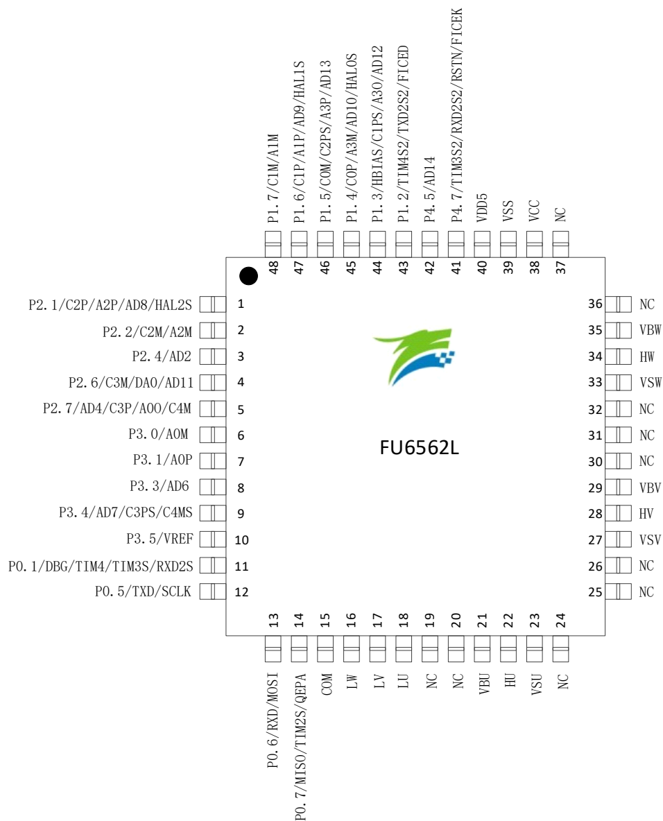
Figure 2-4 FU6562L LQFP48 Pinout Diagram
