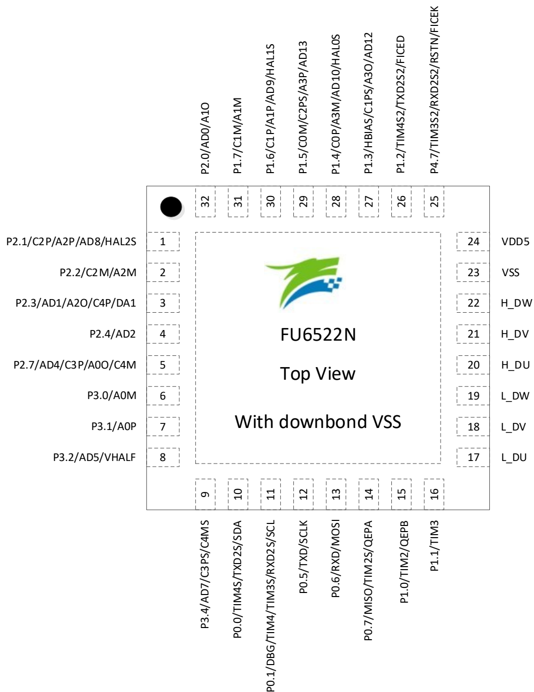
Figure 2-7 FU6522N QFN32 Pinout Diagram
