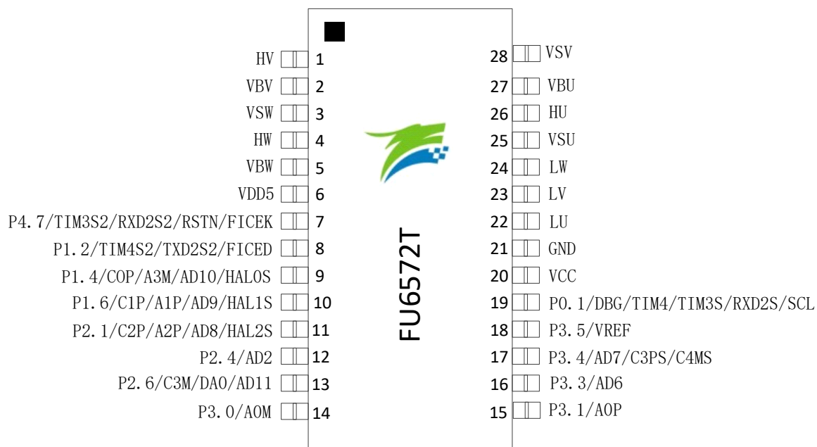
Figure 2-3 FU6572T TSSOP28LD Pinout Diagram
