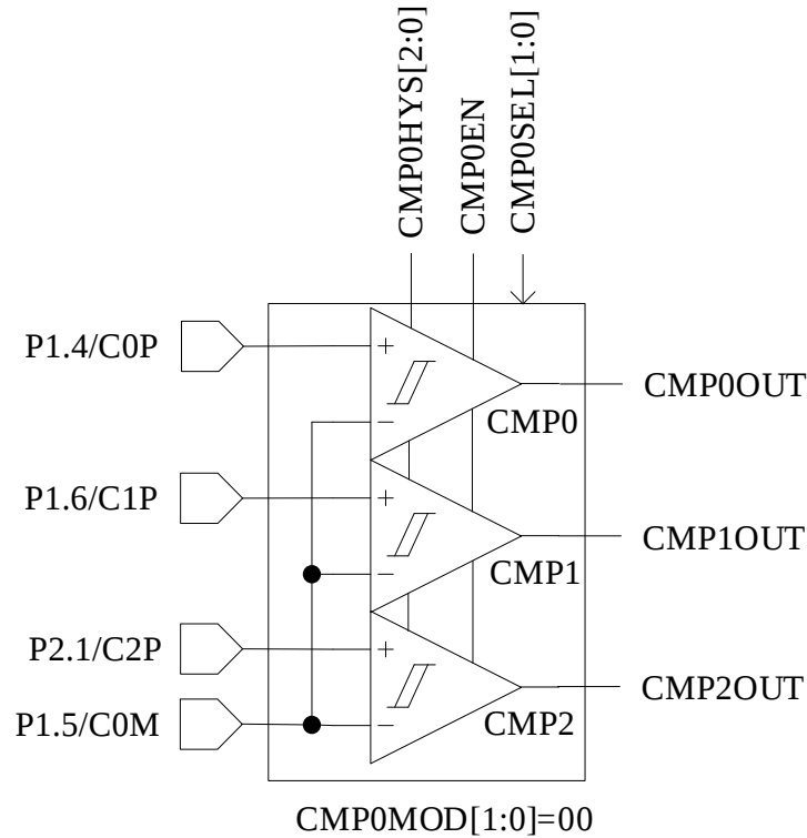
Figure 27-8 CMPG Mode with Built-in Three Comparators
