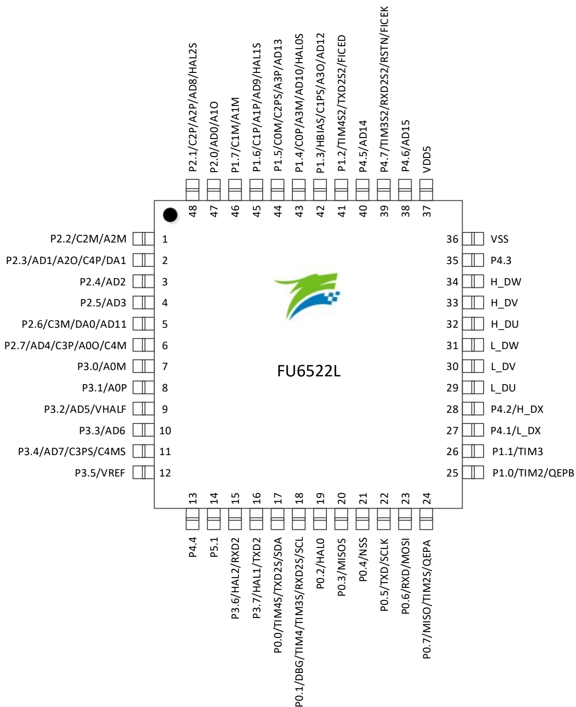
Figure 2-6 FU6522L LQFP48 Pinout Diagram
