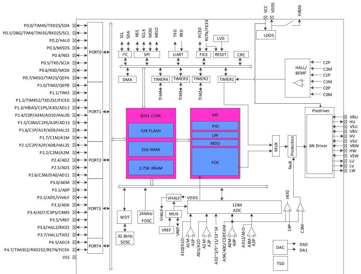
Figure 1-1 Functional Block Diagram of FU6572L
