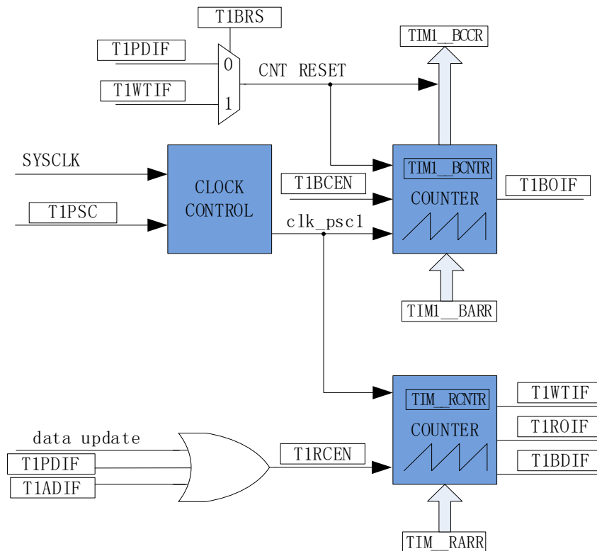
Figure 13-2 Timebase Unit
