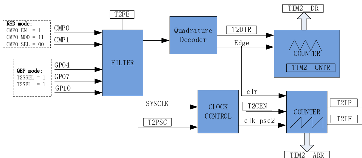
Figure 14-9 Schematic Diagram of QEP&RSD Mode
