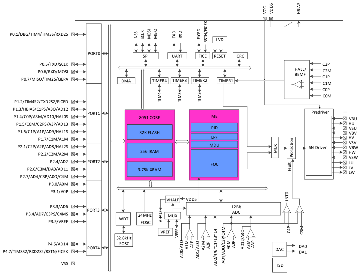
Figure 1-4 Functional Block Diagram of FU6562L
