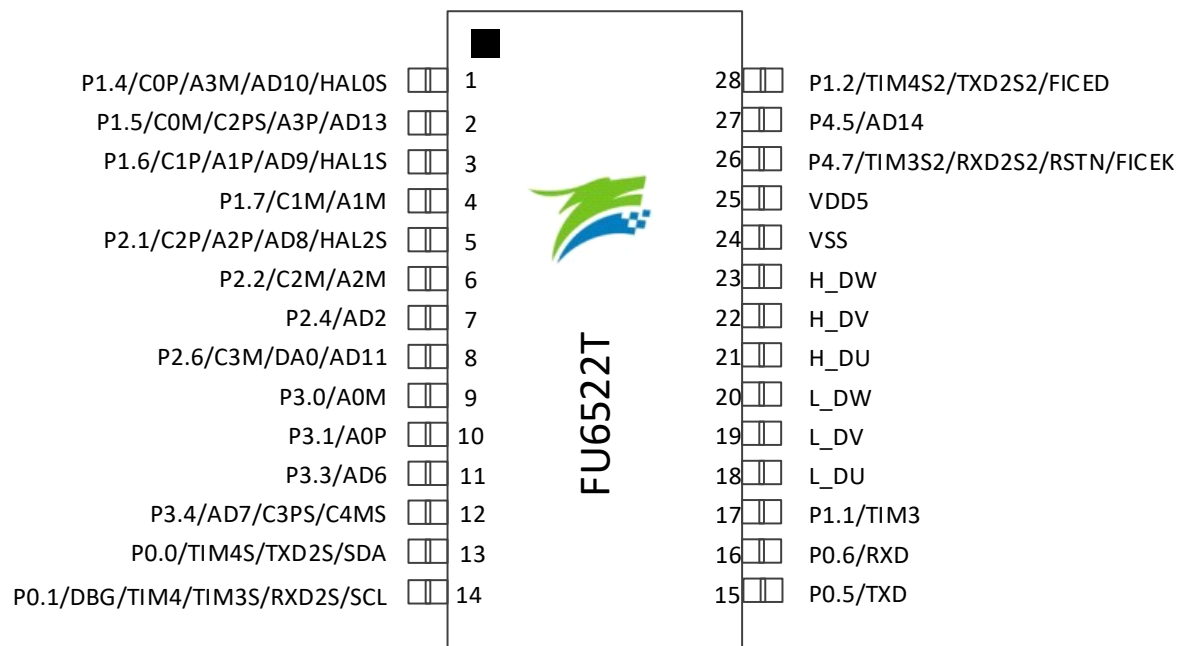
Figure 2-8 FU6522T TSSOP28LD Pinout Diagram
