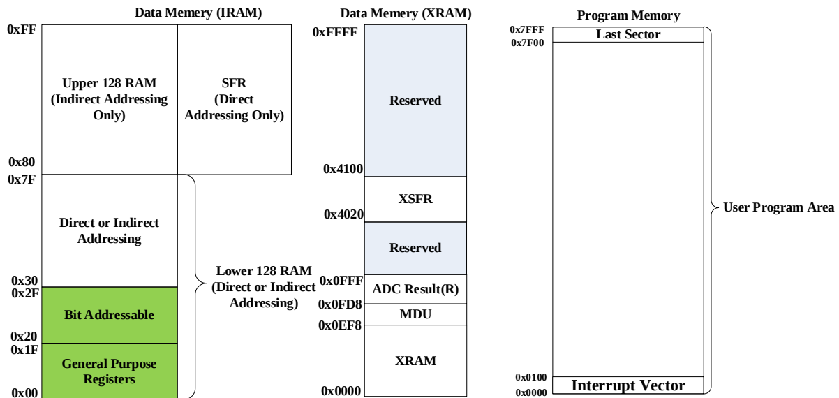
Figure 1-9 Memory Map
