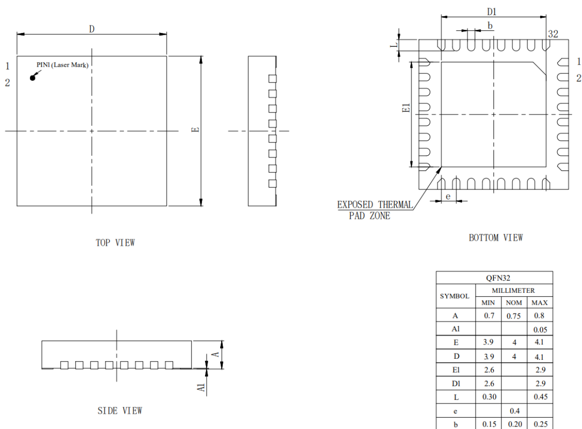
Figure 3-3 QFN32_4X4 Package Drawings and Dimensions
