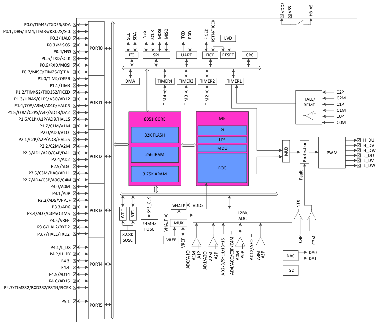
Figure 1-6 Functional Block Diagram of FU6522L
