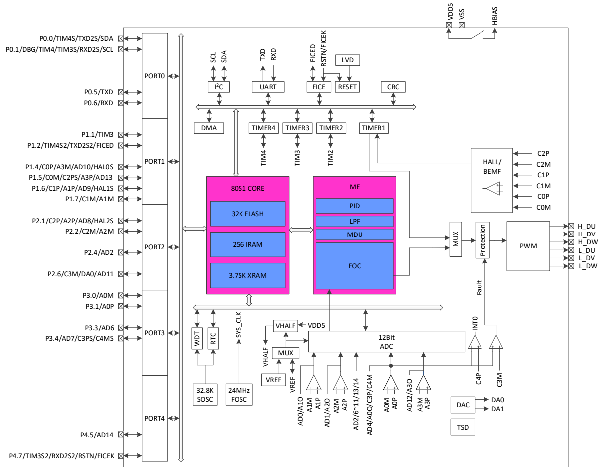
Figure 1-8 Functional Block Diagram of FU6522T
