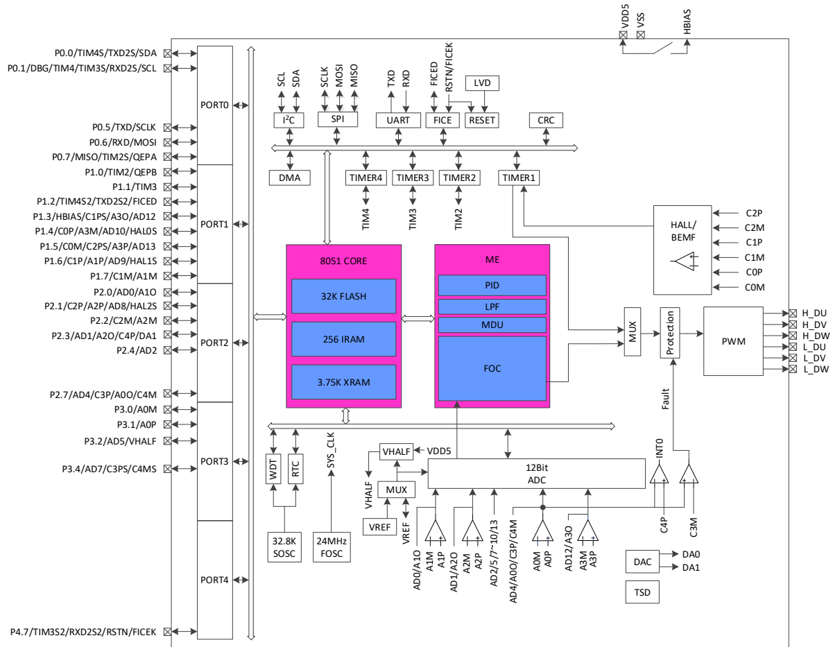
Figure 1-7 Functional Block Diagram of FU6522N
