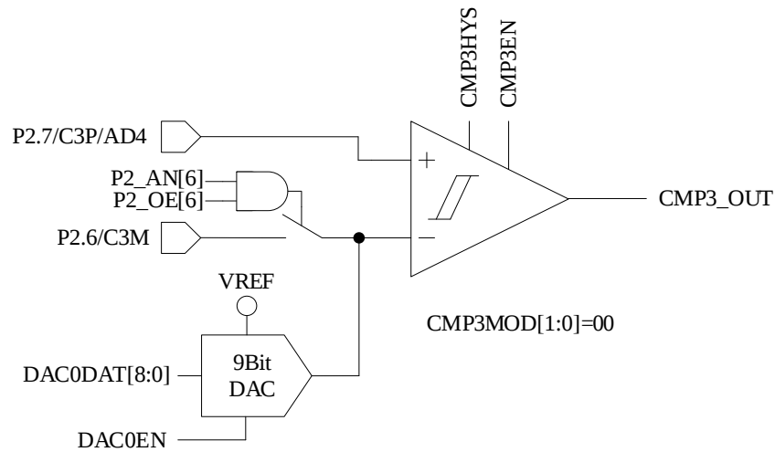
Figure 27-2 Single-comparator Input Mode
