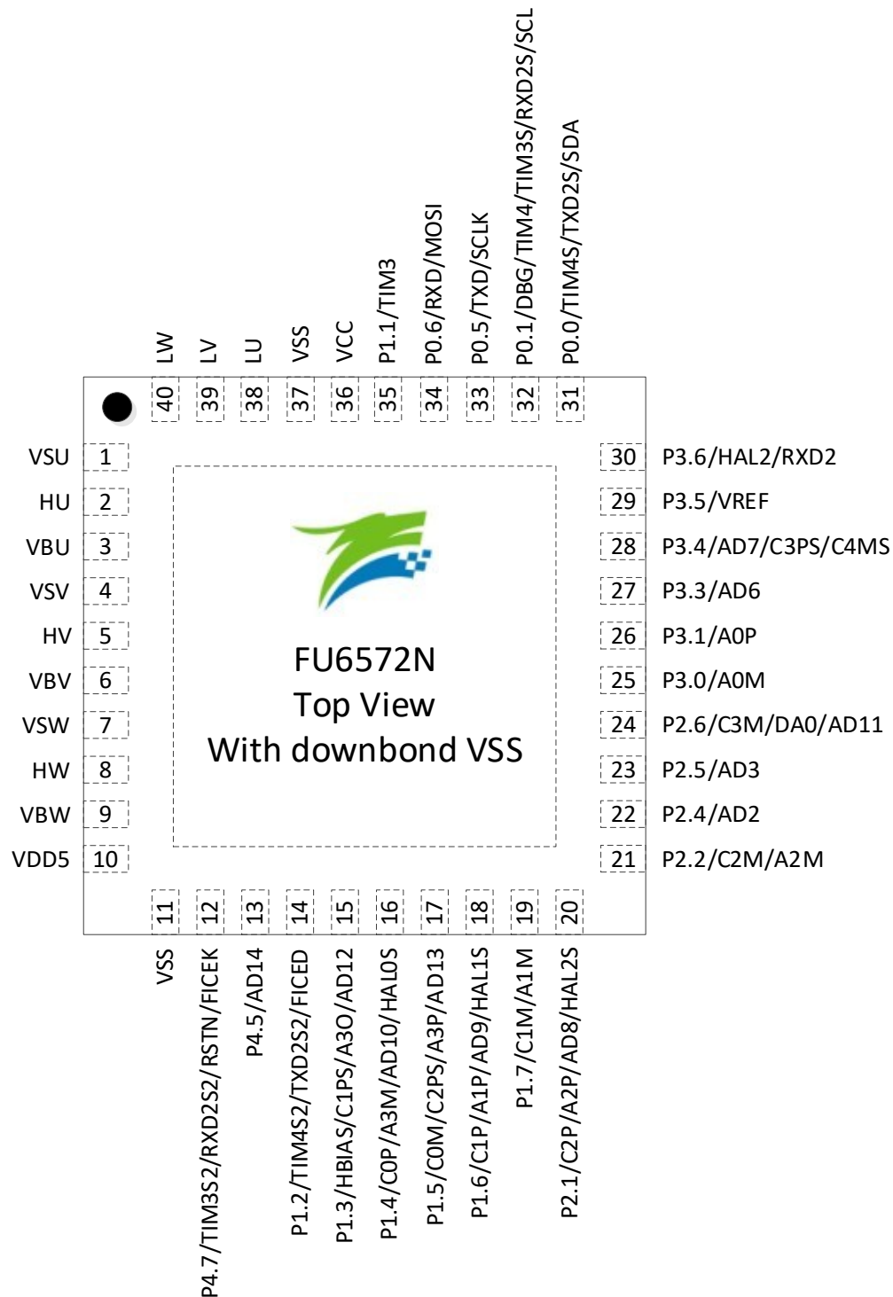
Figure 2-2 FU6572N QFN40 Pinout Diagram
