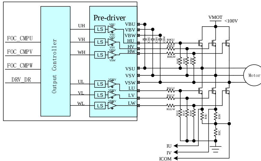
Figure 17-1 Block Diagram of FU6572/FU6562 Driver Module
