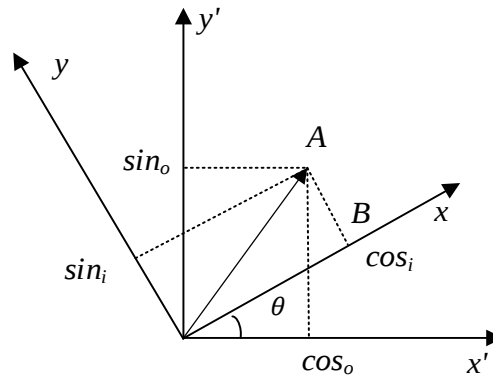
Figure 11-1 Coordinate Transformation
