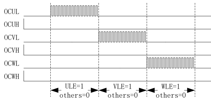
Figure 17-7 Pre-charge Waveform
