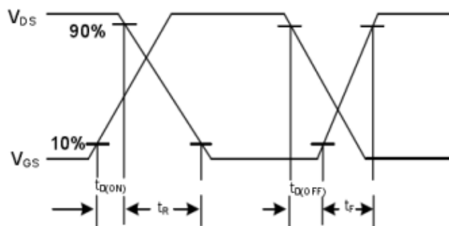
Switching Waveforms
