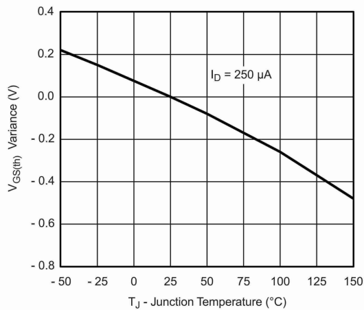
Threshold Voltage Variance Over Temperature
