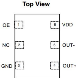
Figure 1. Pin Assignments
