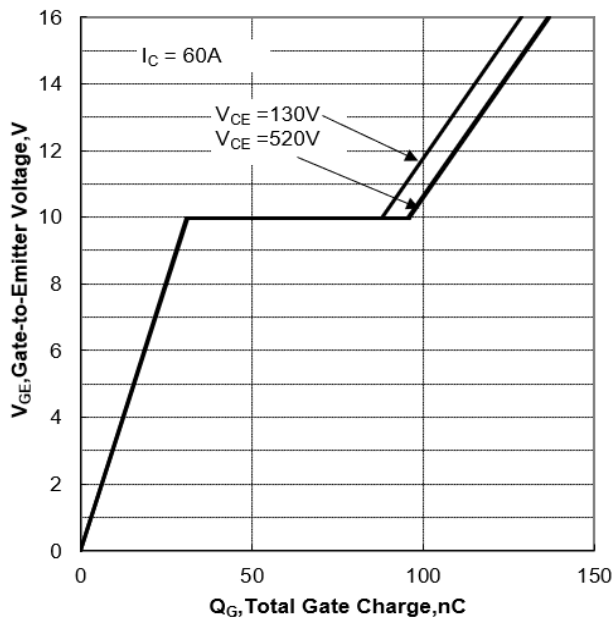
Figure 21. Typical Gate Charge
