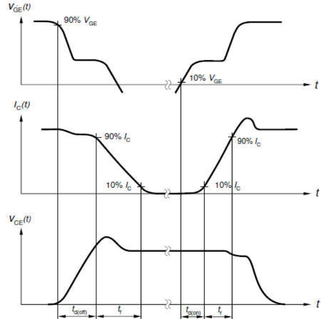
Figure 2. Definition of switching times
