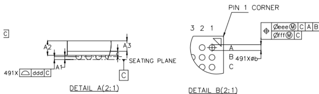
Fig. 2-3 RV1126B PKG Detail A&B
